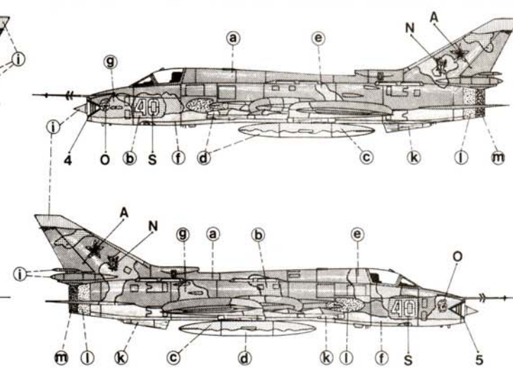
5 Su-17M4 Fitter K, 2nd Sqn, 20th Guards Fighter-Bomber Regiment, 16th Air Army, Russian A.F.; Gross-Dölln A.B., Germany, 1992.
