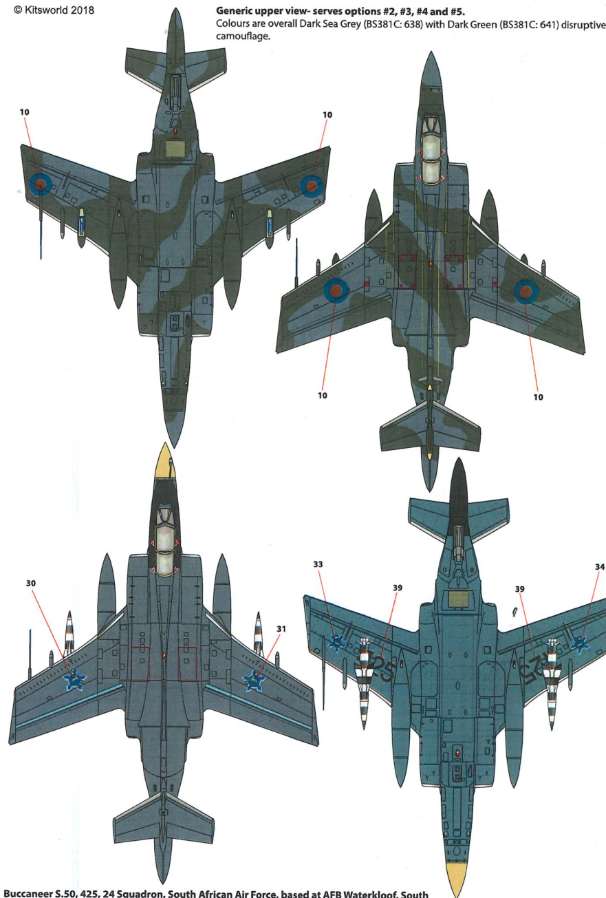
Buccaneer S.50, 425, 24 Squadron, South African Air Force, based at AFB Waterkloof, South Africa, 1966. Dark Sea Grey (BS381C: 638) to the upper surfaces with PRU Blue undersides. The radome is in tan. The aircraft carries two Nord AS.30 anti-ship missiles. The black and white banding denotes a training round.
