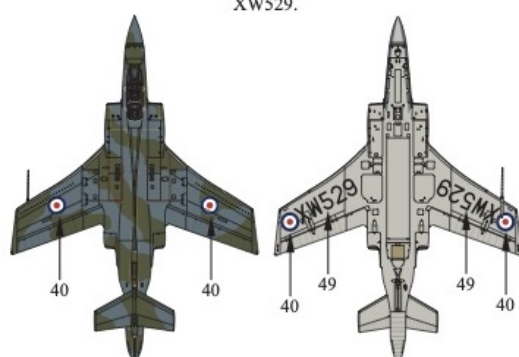
Hawker Siddeley Buccaneer S.2 XW529.
