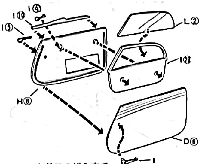
29 左ドアの組み立て Apply cement to inside of I 20 lightly and press window in place. Be sure not to smear clear parts. Cement trim to door and door sections over I 20.
