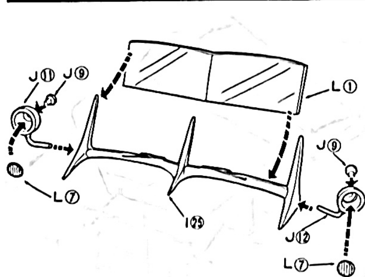
31 ウィンドシールド部の組み立て Cement windshield and lamps to frame. Apply cement sparingly to clear parts to avoid discoloration.
