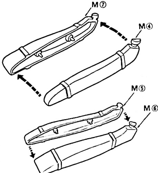
45 補助タンクの組み立て Cement auxiliary tanks together as shown.
