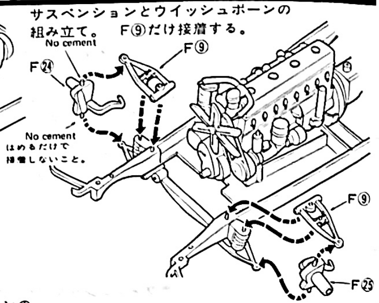
10 Cement suspension wishbones F(9) to the chassis over front axle stubs. Do not allow cement to touch the pins on the stubs.
