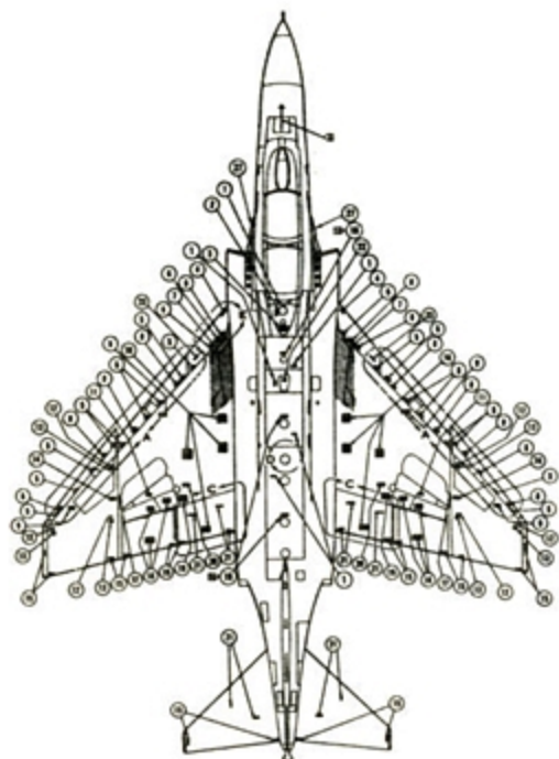
FUSELAGE TOP
