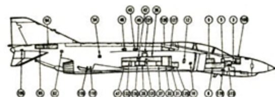
ACCESS DOORS RIGHT SIDE
