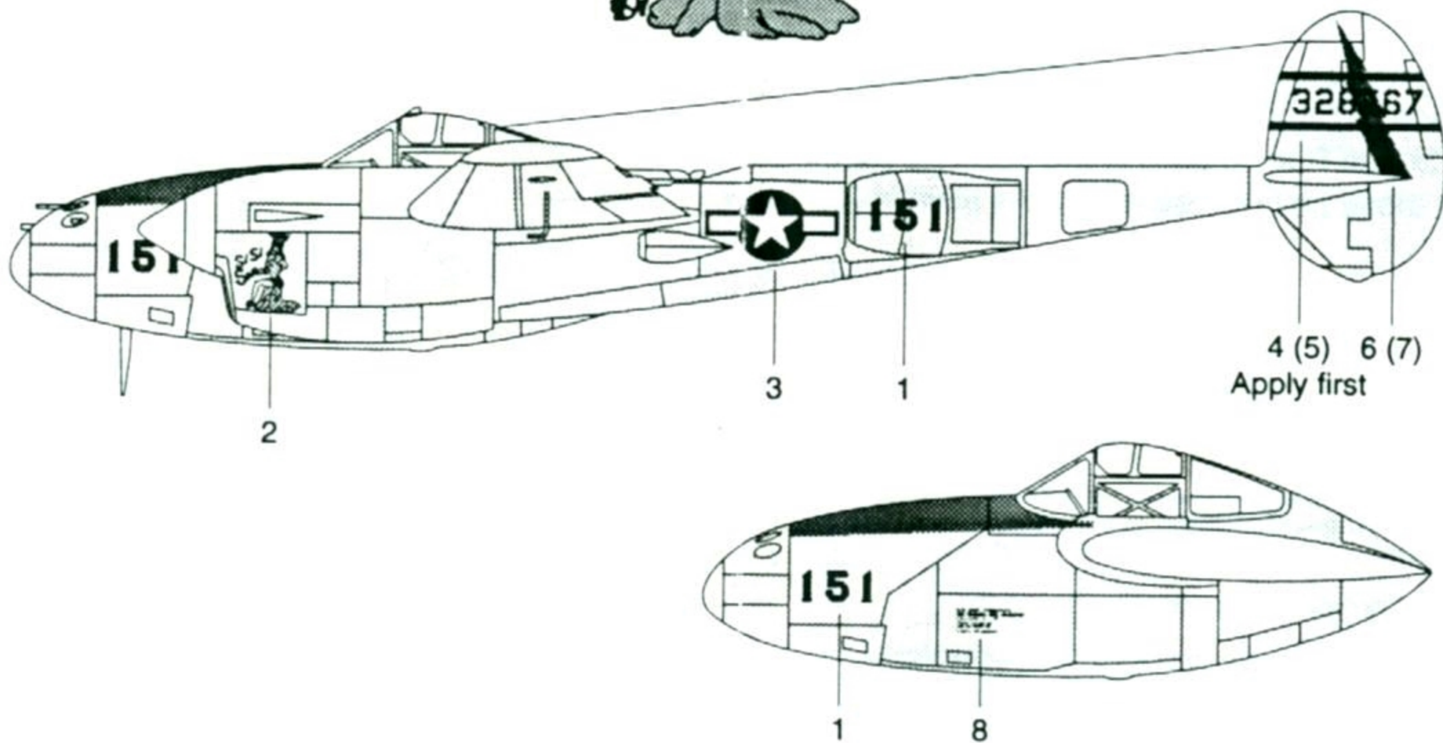
P-38J-15-LO, 43-28767, "Si Si Señor", 67th Fighter Squadron, 347th Fighter Group, XIII Air Force, Philippines, 1945. Flown by Maj. Bill Walling. Overall natural metal finish with yellow spinners, inner and outer vertical stabilizer tips, and top and bottom horizontal stabilizer tips. Standard olive drab anti-glare panels. Open spoked wheels had natural metal hubs. Note that decals 6 and 7 are applied over the serial numbers and black stripes.
