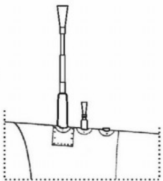
WEAPON CONFIGURATION USED ON SOME F6F-5N NIGHTFIGHTER:
