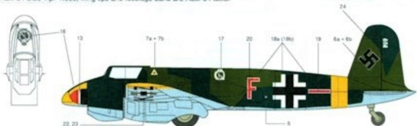
Hs 129B-1/R-2, 8.Sch. Gr. 1, Russian Front, Summer 1943. RLM 70 Schwarzgrün and RLM 71 Dunkelgrün upper surfaces with RLM 65 Hellblau beneath. Spinner is RLM 70 Schwarzgrün or black with a RLM 23 Red Tip. Nose, wing tips and fuselage band are RLM 04.
