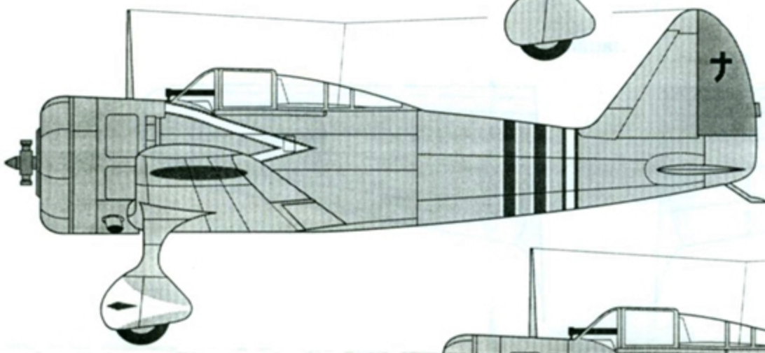
Nakajima Ki-27b, 77th Air Combat Regiment, Headquarters Company, Meshod, Thailand, 1941. Overall IJAAF green-grey. Aircraft shot down by a member of the American Volunteer Group "Flying Tigers" in December 1941.
