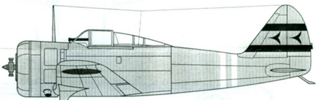
Nakajima Ki-27b, 77th Air Combat Regiment, Headquarters Company, Meshod, Thailand, 1941. Overall IJAAF green-grey. Aircraft shot down by a member of the American Volunteer Group "Flying Tigers" in December 1941.
