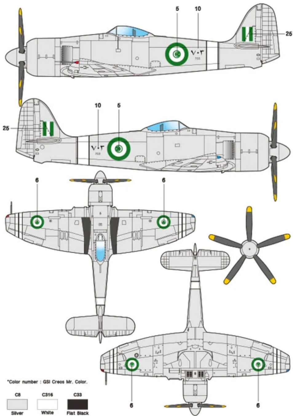
1. Hawker Sea Fury FB.11, 703, Royal Egyptian AF, 1966
