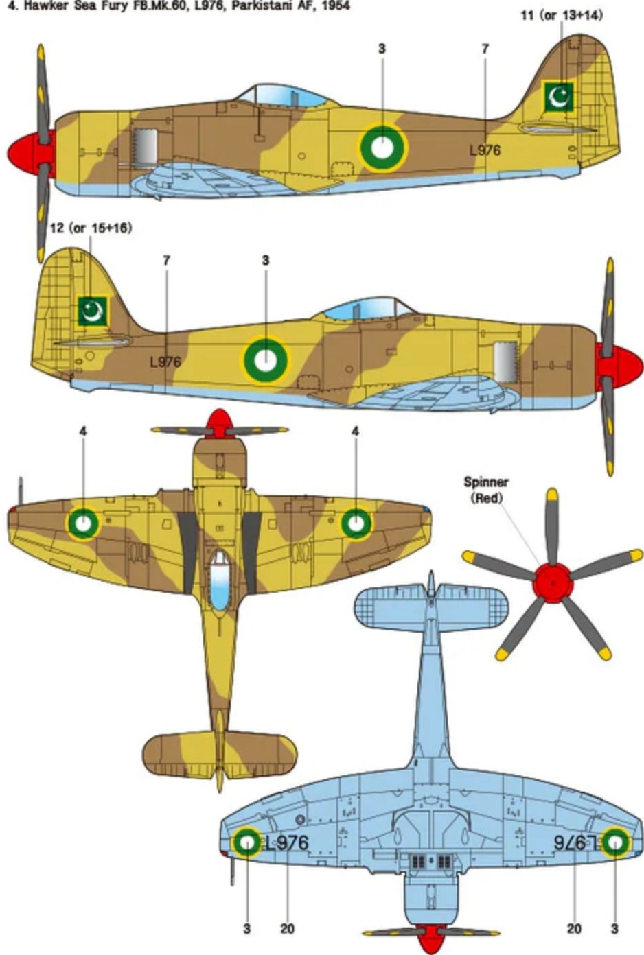
4. Hawker Sea Fury FB.Mk.60, L976, Parkistani AF, 1954
