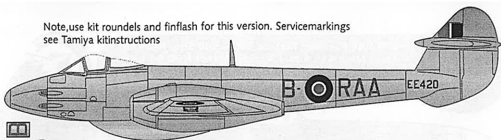
Meteor F.Mk.3. RAA B. EE420. No.500 Sqn. RAuxAF. West Malling 1950. Overall 'High Speed' Silver finish. Recommended kit: Tamiya F.3
