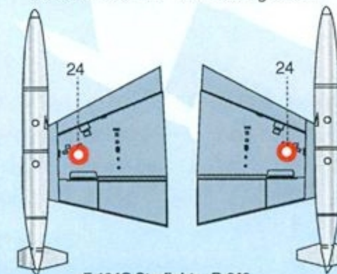
F-104G Starfighter R-346 Scrap view of wing under surfaces
