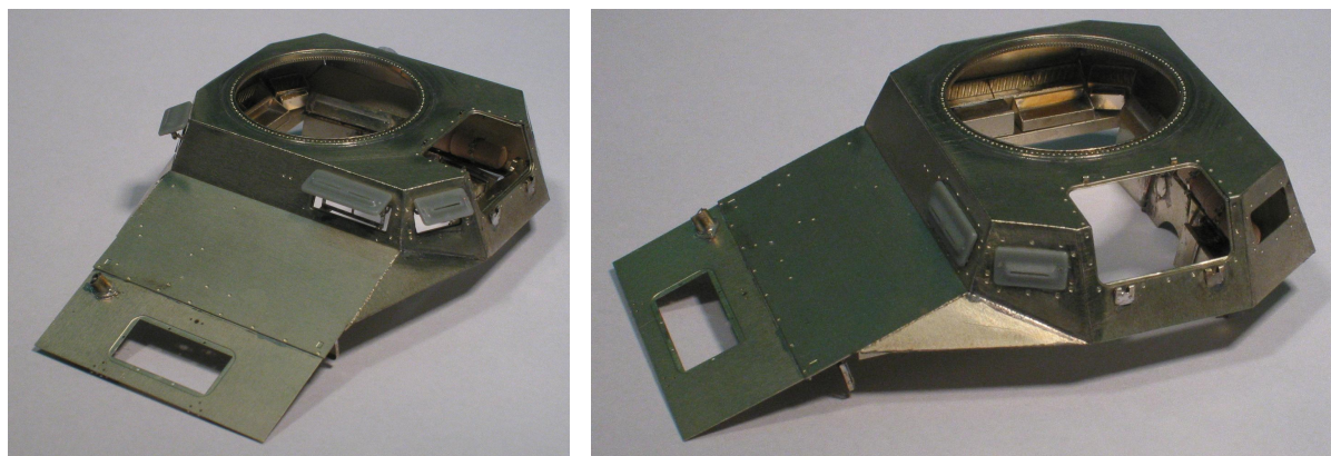
Reworked part 1 from set 35 066 Pz.Kpfw. I A Upper hull (prerobiona część nr1 z 35 066)
