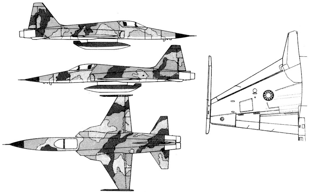
F-5E(74-00959)"CHUNG CHENG" of 2nd Fighter Wing of Nationalist Chinese Air Force, Taiwan. National Insignia on upper wings only. USAF Standard Camouflage scheme with underside.
