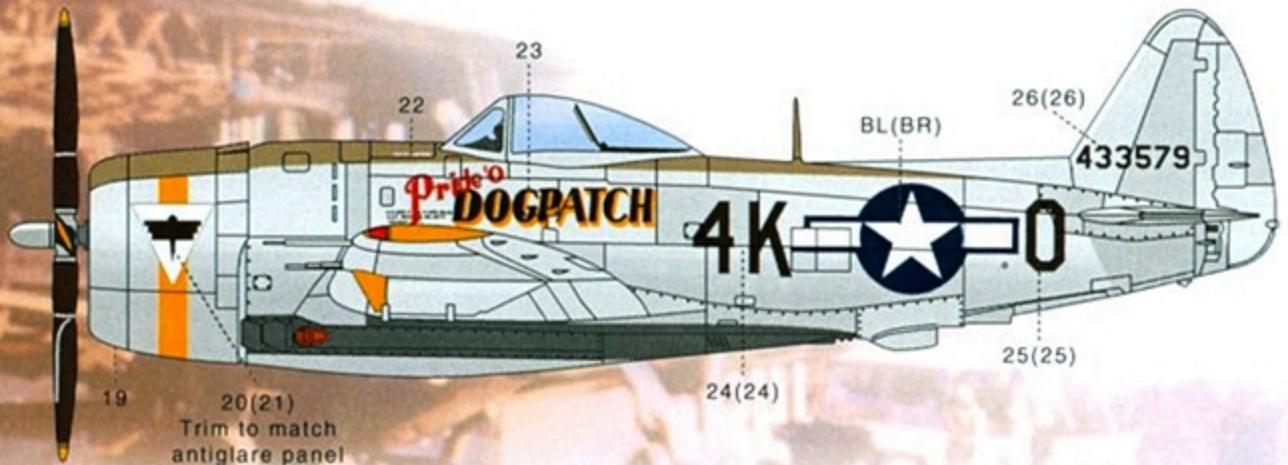
Aircraft 4 - P-47D-30-RA, 'Pride O' Dogpatch' flown by Lt. Harry H. 'Pappy' Yokum, 506FS, 404FG. Overall natural metal finish with Olive Drab antiglare panel. Curtiss Electric 13'1" asymmetrical propeller with unpainted prop hub. Black belly paint. Yellow wing tips and forward pylons. Trim decals 20/21 to match painted antiglare panel.
