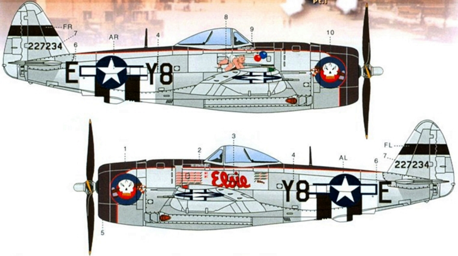
Aircraft 1 - P-47D-27-RE 'Elsie/Lil Butch', flown by Major Clay Tice, Squadron Commander of 507FS, 404FG. Overall natural metal finish with customized Black antiglare panel. Black tail bands. Partial invasion stripes on fuselage. Note oversized and doubled underwing insignias. Use Red decal stripes provided to border antiglare panel. H.S. propeller. No data block on this A/C.
