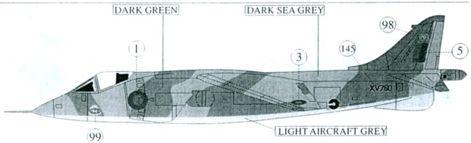
HARRIER GR.1, n. 233 Operational Conversion Unit, Wittering 1971
