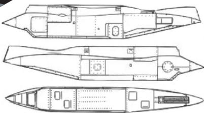
Type «D» POD (suitable for Mig-21R all model kit)
