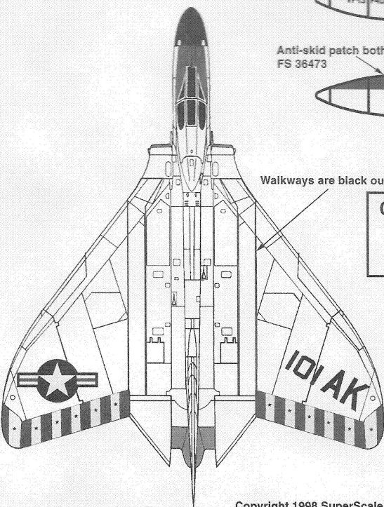
Top View VF-13
