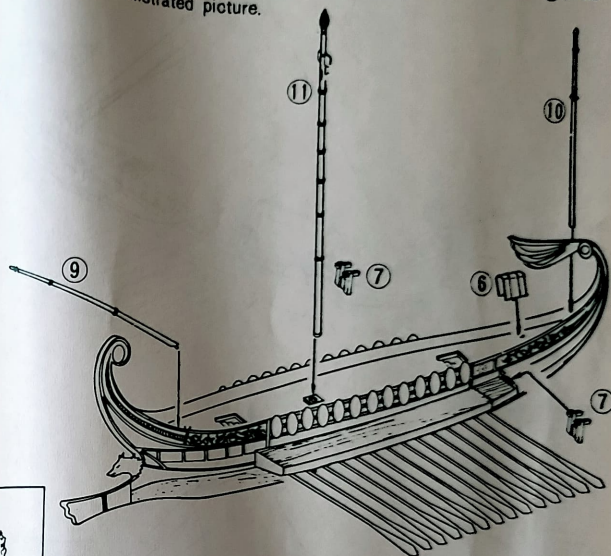
Plan of complete ship
