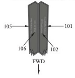
Front Nose Gear Doors
