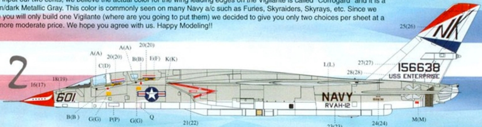
RA-5C Vigilante BuNo. 156638. The Speartips of RVAH-12 were aboard USS Enterprise (CVAN65) for the last war cruise of the Viet Nam War in April, 1975. Non-specular Gull Gray FS36440 upper surfaces with Gloss White FS17875 vertical tail, undersides, control surfaces, landing gear, wheel wells, and fin tip antenna. Wing leading edge slats Dark Gull Gray FS35231; radome and edges of gear doors FS11136 Insignia Red.
