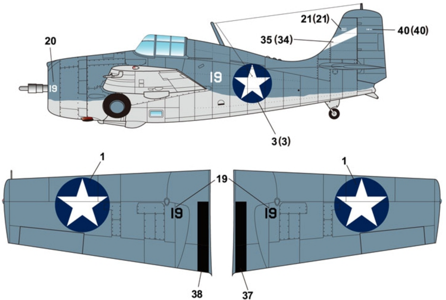
4. F4F-4 BuNo. 03417/white 19, flown by Lt Stanley Winfield ('Swede') Vejtasa, VF-10, USS Enterprise, 26 October 1942
