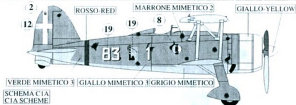
Fiat CR42 MM. 5667 , 83 o Sq.18 o Gr.56 o St.C.T.Cap.Molinari, Ursel (Belgium) November 1940
