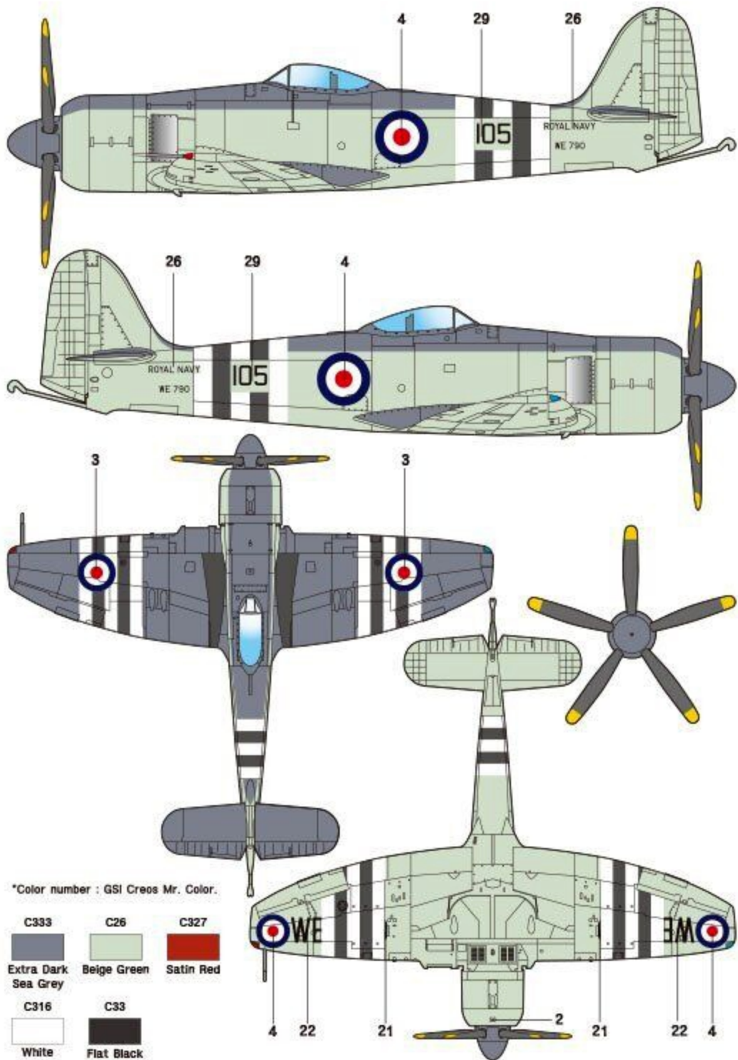
3. Hawker Sea Fury FB.11, No.105, VE790, 808th Squadron, HMAS Sydney, Korea, 1951 Oct. ~ 1952 Jan.
