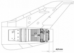
R11P-380 engine flame holder part correct installation (view from rear)
