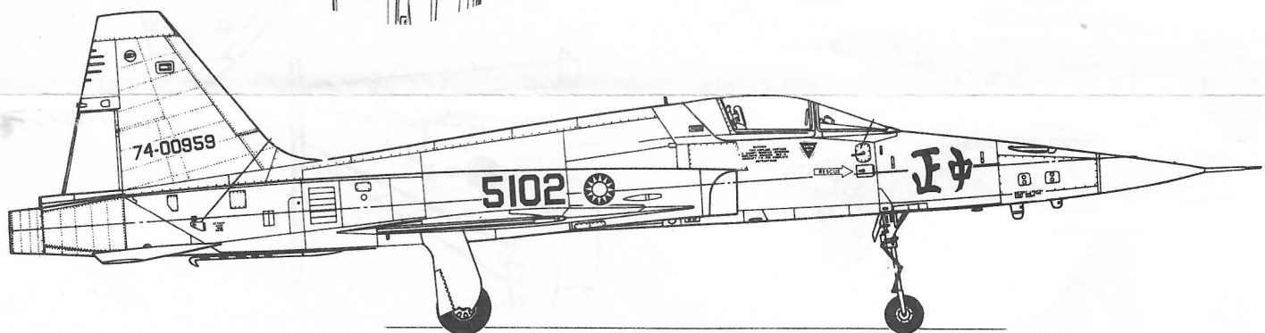
F-5E(74-00959)"CHUNG CHENG" of 2nd Fighter Wing of Nationalist Chinese Air Force, Taiwan. National Insignia on upper wings only. USAF Standard Camouflage scheme with gray underside.
