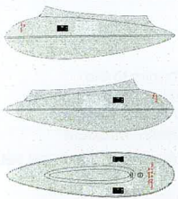
Scheme 3
