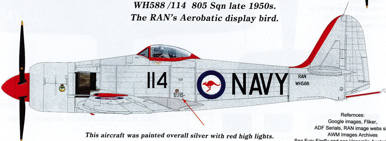
Scheme 6
