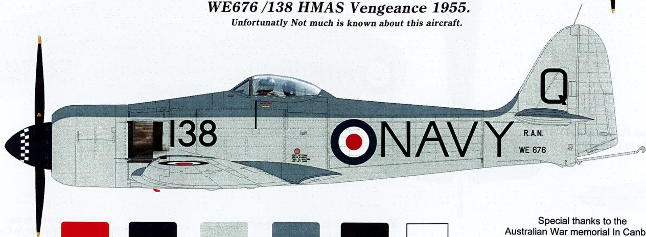
Scheme 3
