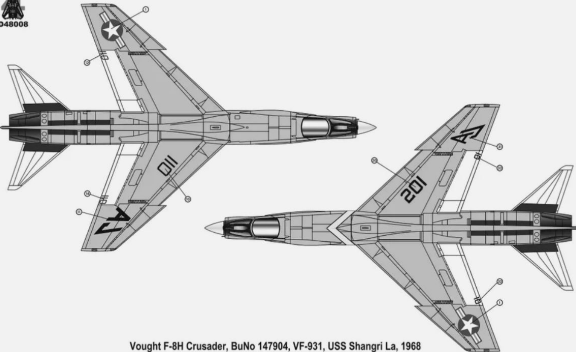
Vought F-8H Crusader, BuNo 147904, VF-931, USS Shangri La, 1968
