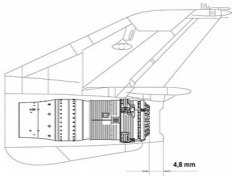
R11F2-300 engine flame holder part correct installation (view from rear)
